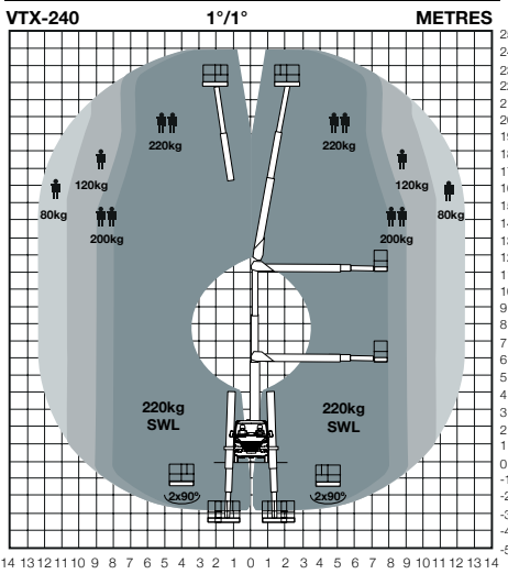
Working envelope at 80/120/200/220kg bucket SWL
